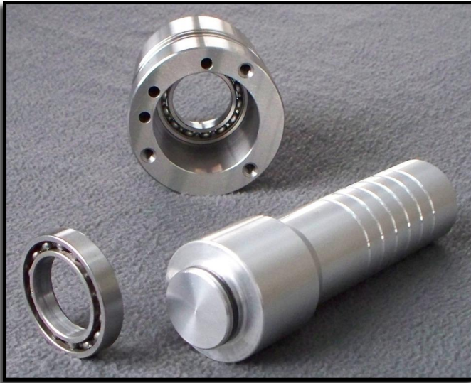
T-3600AC pictured with a new bearing. An OEM center support hub is placed in the background for reference.
